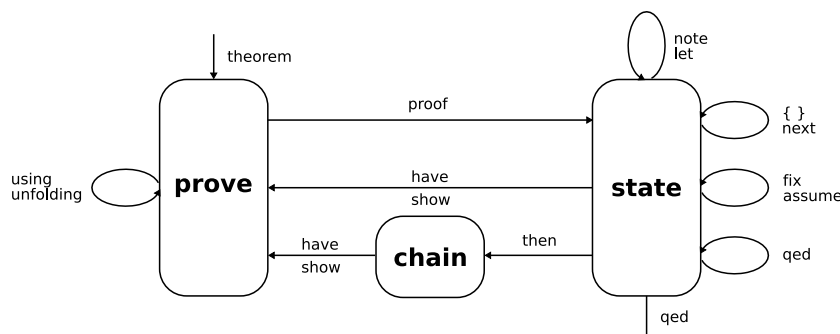
Figure 2.2: Isar/VM modes
