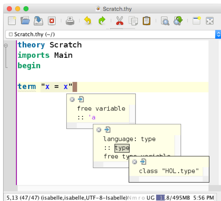
Figure 3.7: Nested tooltips over formal entities
