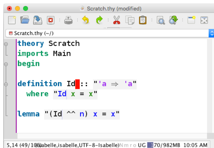
Figure 3.9: The result of semantic selection and systematic renaming
