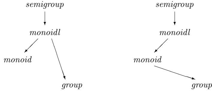
Figure 1: Subclass relationship of monoids and groups: before and after establishing the relationship \text{group} \subseteq \text{monoid} ; transitive edges are left out.
