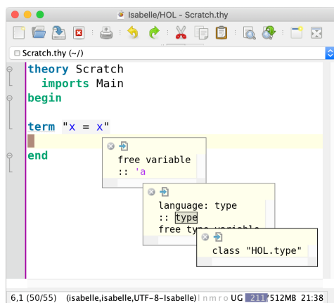
Figure 3.7: Nested tooltips over formal entities
