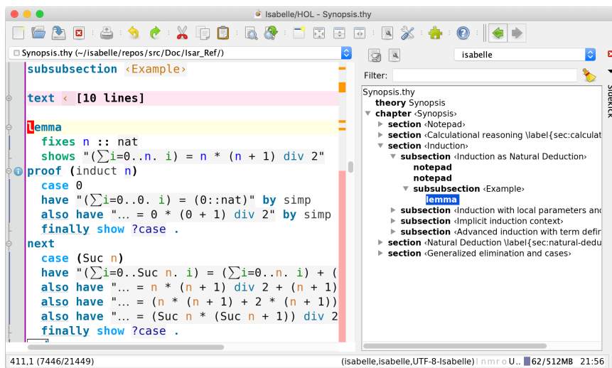
Figure 4.1: Isabelle document outline via SideKick tree view
