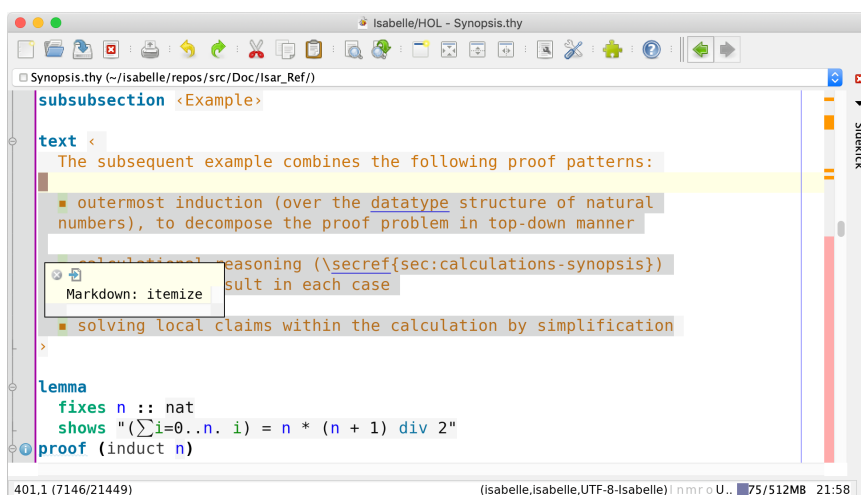
Figure 4.2: Markdown structure within document text
