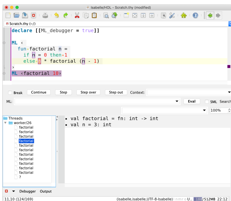
Figure 5.1: ML debugger session
